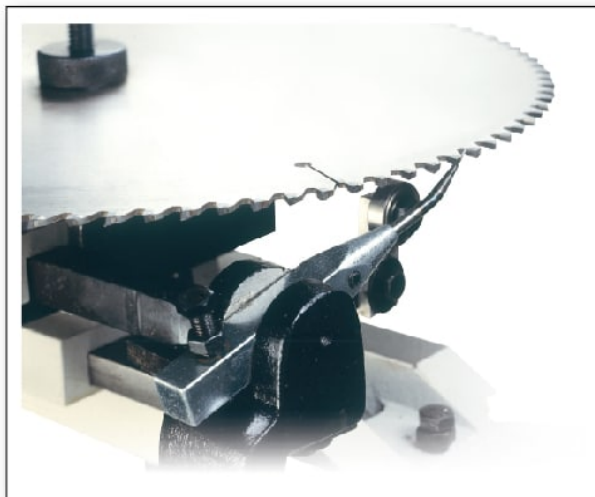
Saw Blade Tip Positioning Device 鋸片頂齒定位裝置
